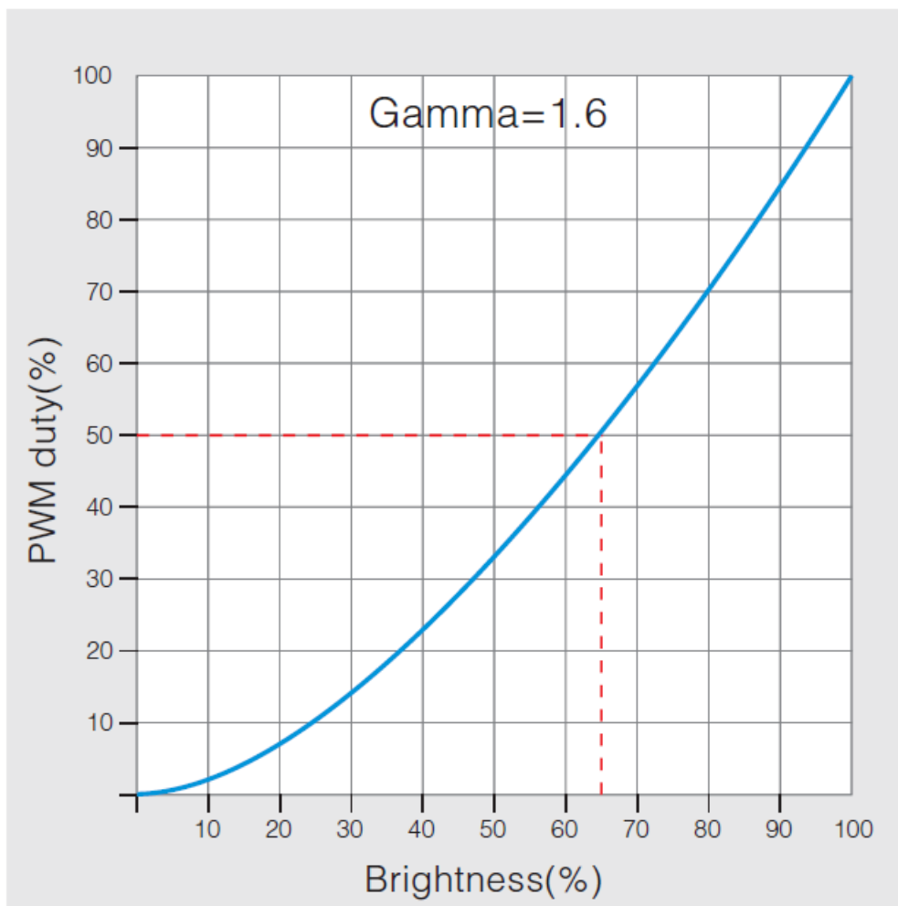
Linear dimming curve
