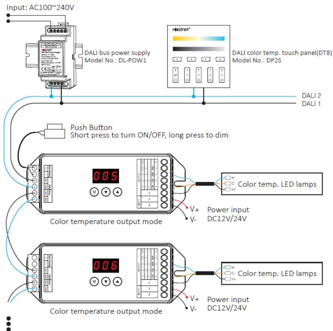
Connection Diagram (Single color output mode)
