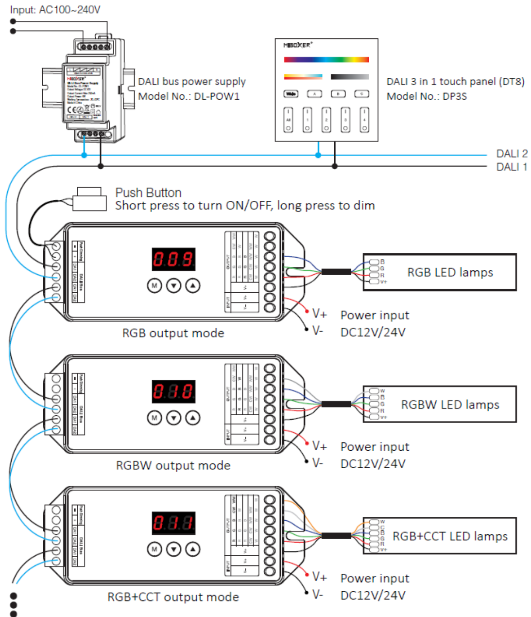
Connection Diagram (Color temperature output mode)
