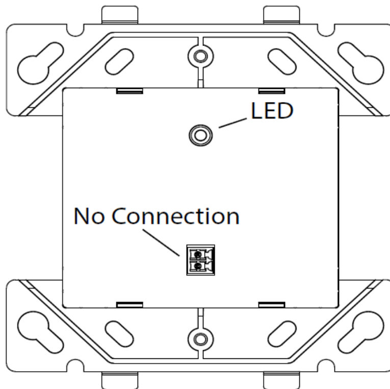
FIGURE 2 MODULE MOUNTING:
