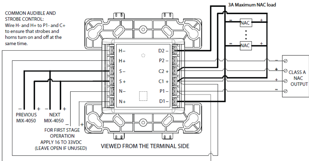
FIGURE 4 DUAL CLASS B WIRING:
