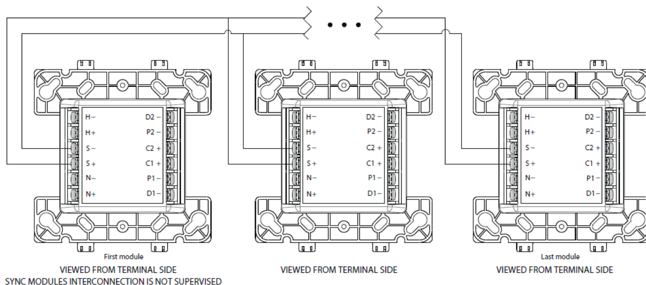
FIGURE 5 SYNC MODULES INTERCONNECTION (20 MODULES MAXIMUM):
