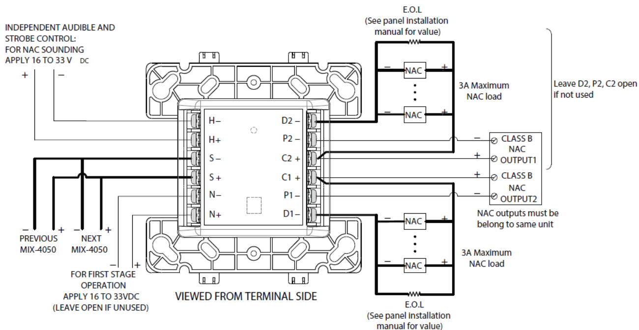
FIGURE 5 SYNC MODULES INTERCONNECTION (20 MODULES MAXIMUM):
