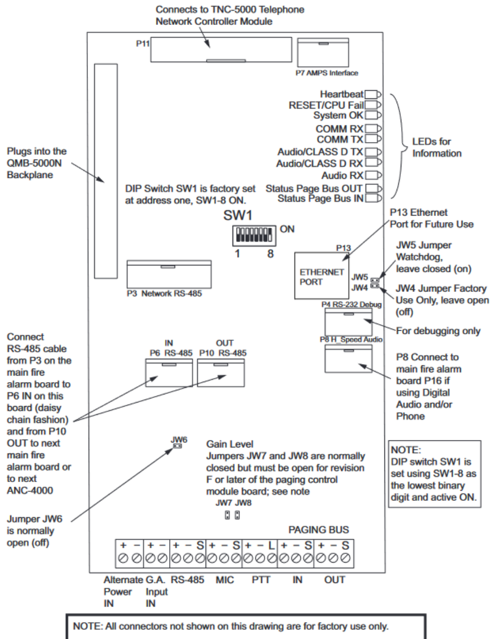
Figure 5: ANC-4000 Audio Network Controller board
