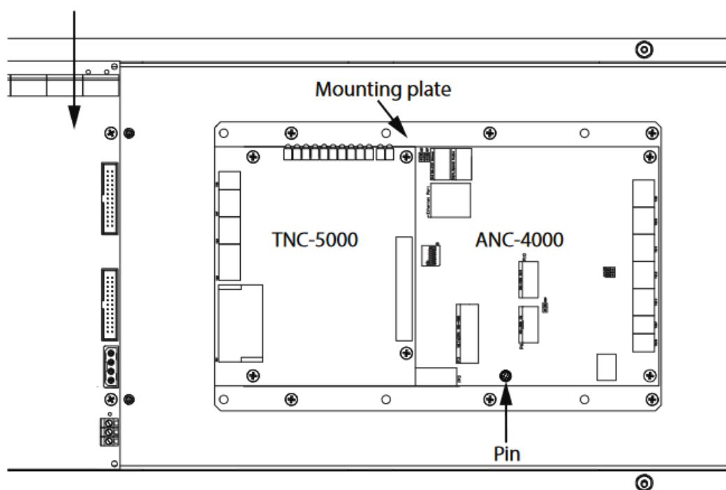
Figure 4: Final Position of ANC-4000, TNC-5000, Mounting Plate
