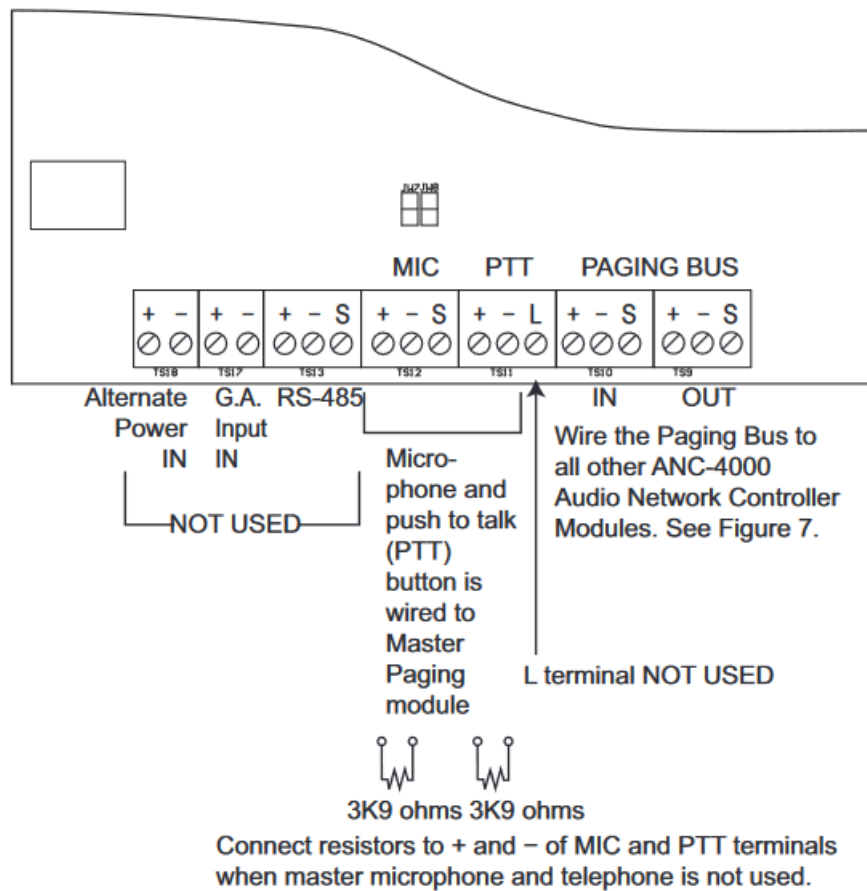
Figure 6: ANC-4000 Wiring Diagram
