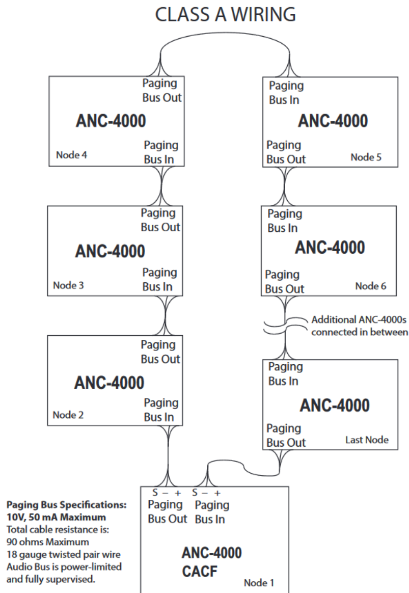
Figure 7: Audio Paging Bus Wiring
