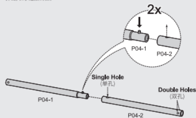
Extended Metal Tube (加长款-金属管)
