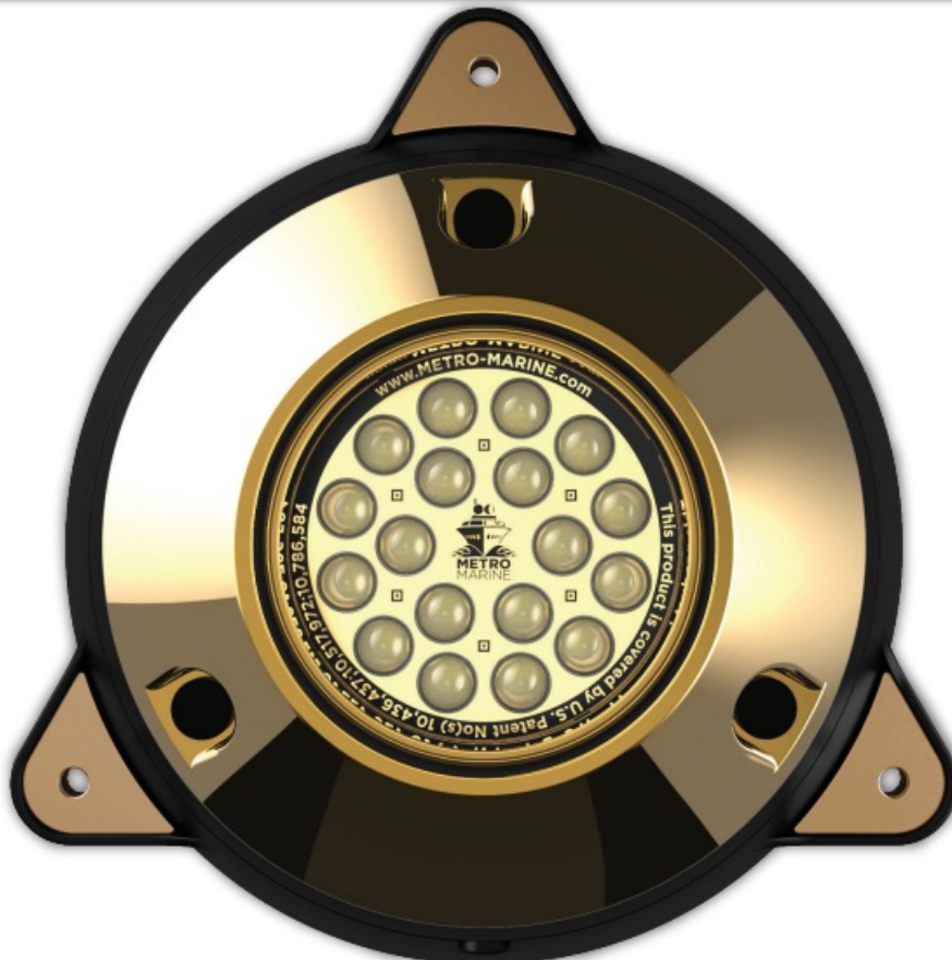
F-Series Single Color Round Fixture F-SMR1-W3-45
