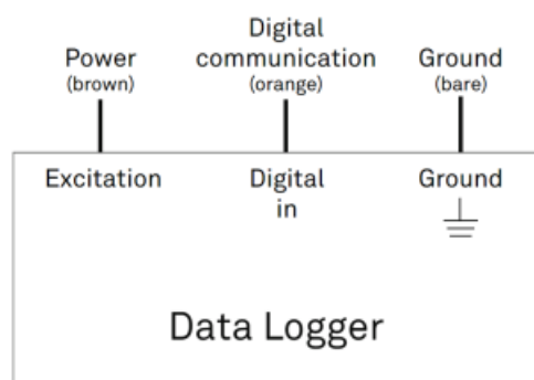
Figure 2 Equivalent circuit diagram
