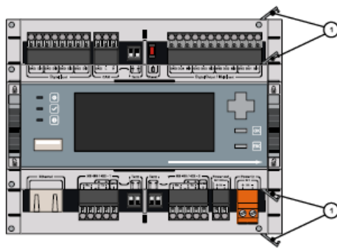
Fig. 4: Unlocking the fasteners
