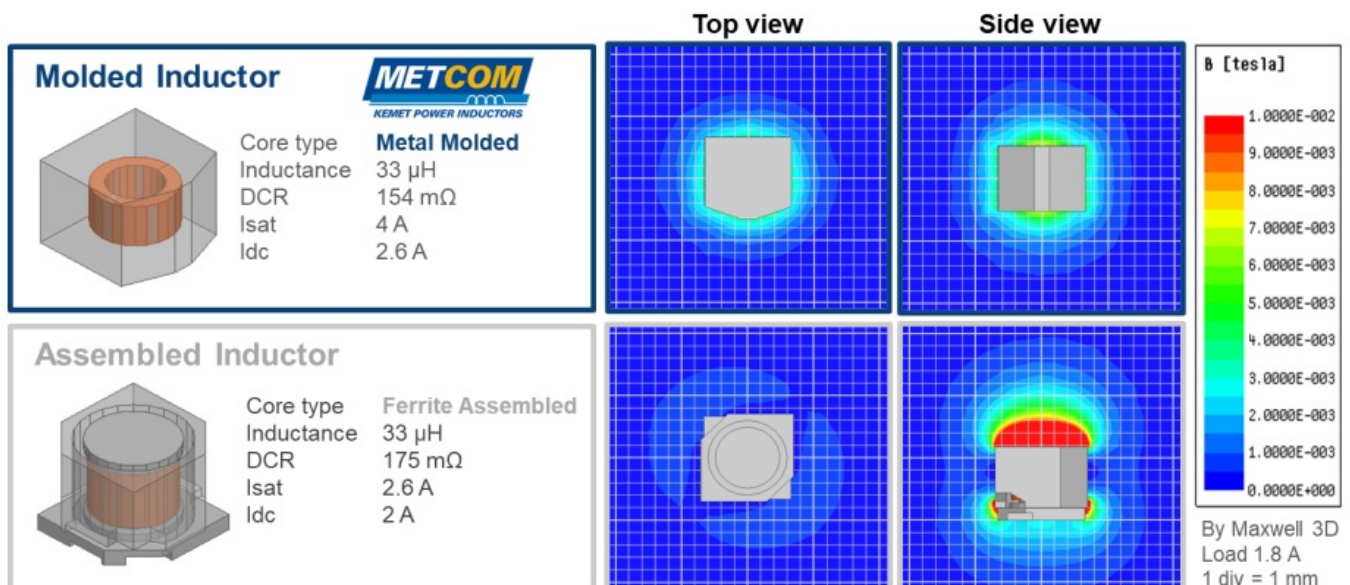
Figure 9 – Magnetic Flux Leaking Amount Comparison
