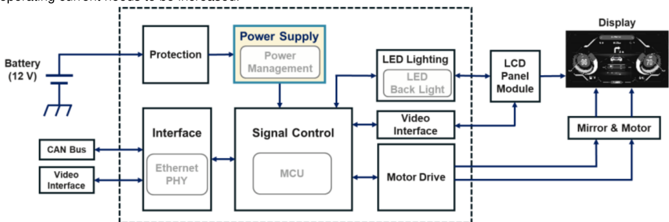
Figure 6 – Block Diagram of the IVI Fourth Stage
