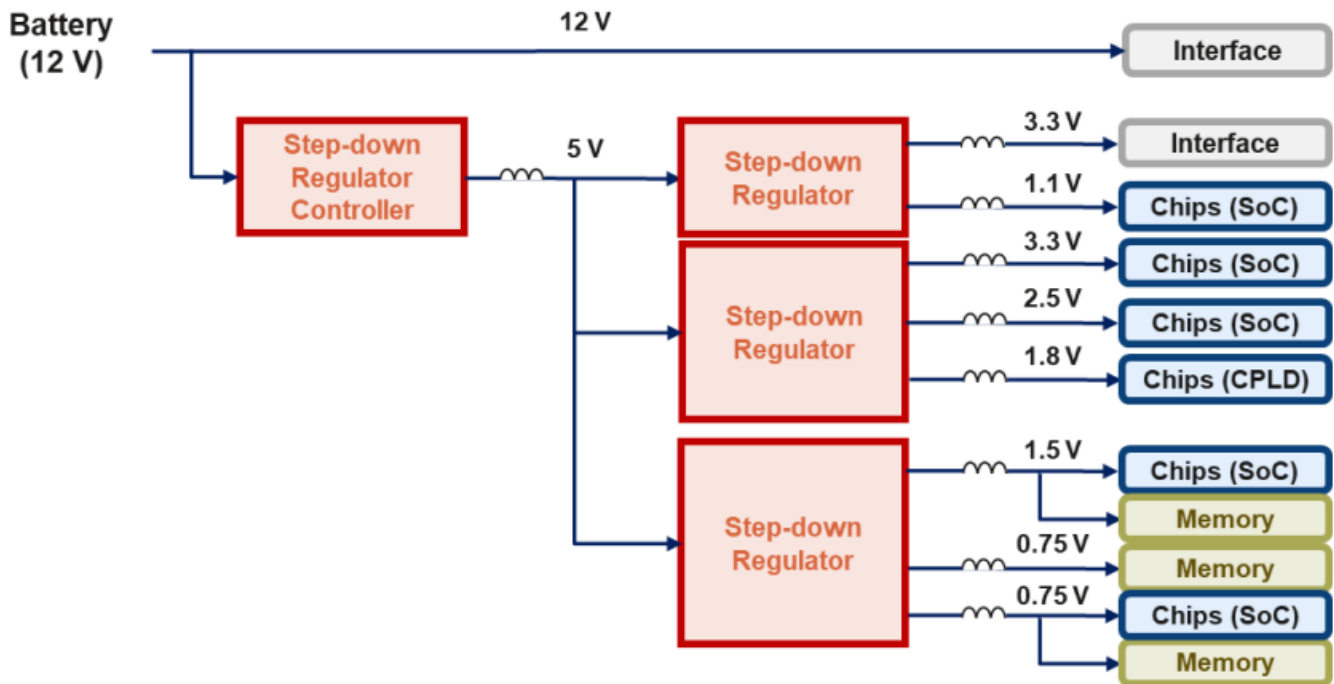
Figure 7 – Power Management System Circuit Design Example
