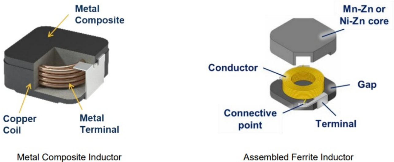
Figure 8 – Inductor Structure Comparison
