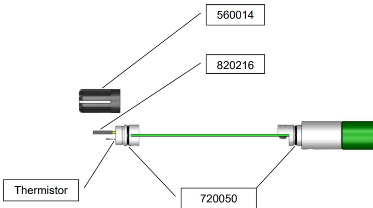
Figure 5 Spare Parts
