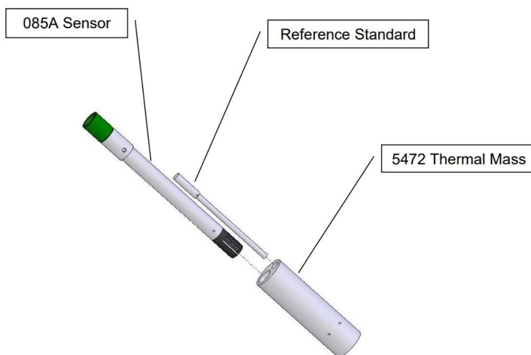
Figure 4 - 5472 Thermal Mass
