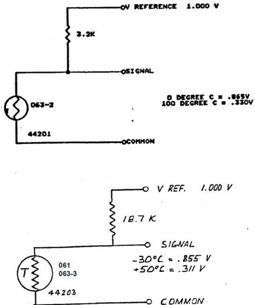
Figure 2-1 Connections of 061/063 Temperature Sensor To Datalogger
