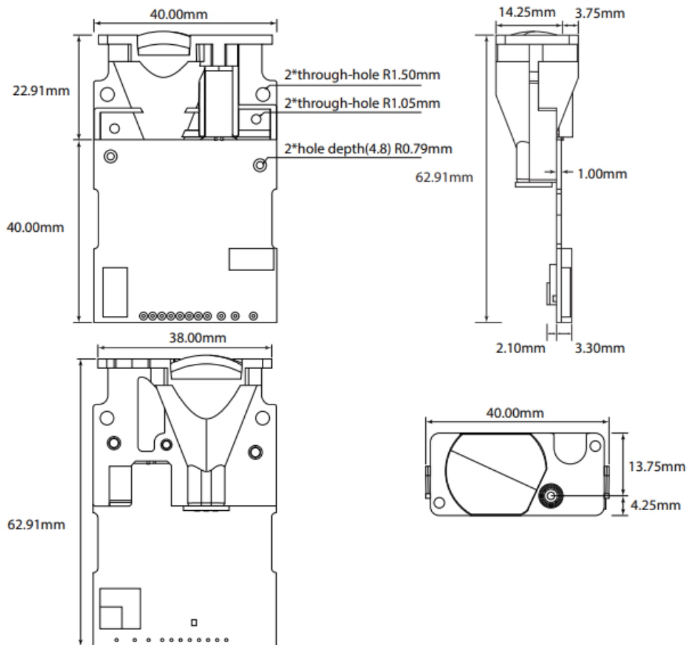
Figure 2-1 Module Overview
