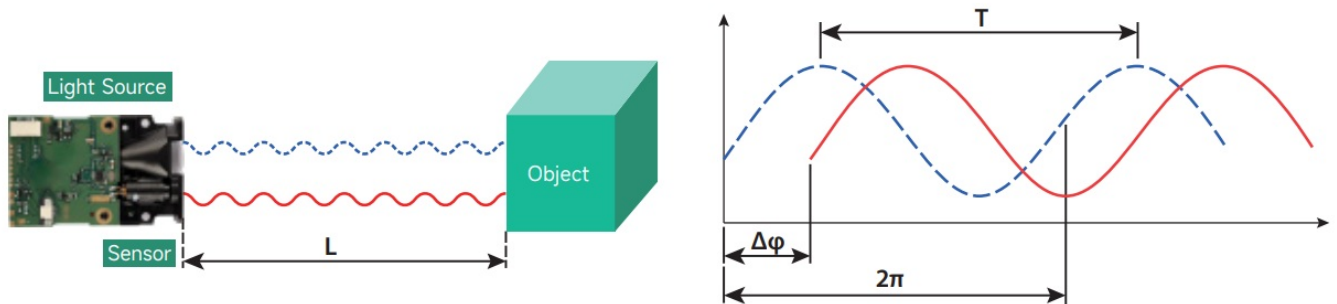
Figure 1-1 Basic Schematic Diagram of Laser Module
