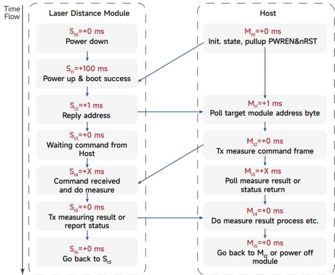
Figure 10-1 Module Communication Timeline
