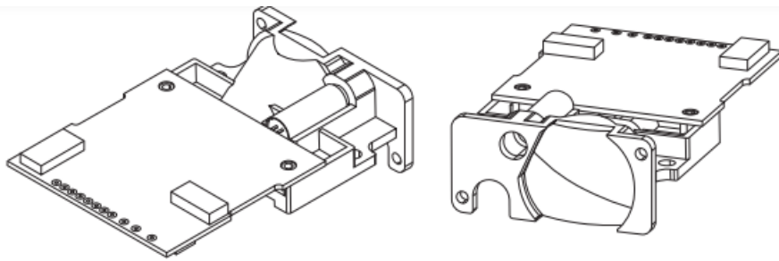
Figure 2-1 Module Overview
