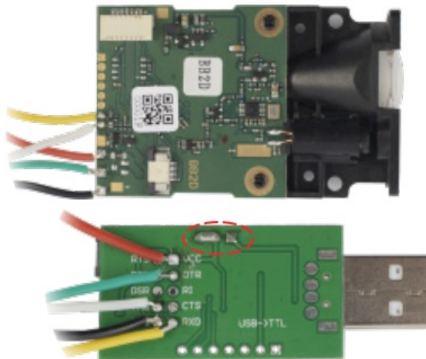
Figure 5-2 Soldering
