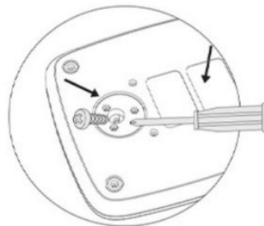
2. Fasten screws on the base to secure.
