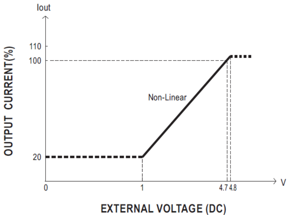
EXTERNAL VOLTAGE (DC)
