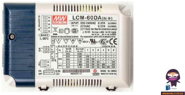
MEAN WELL LCM-60DA Series Multiple Stage Constant Current Mode LED Driver
