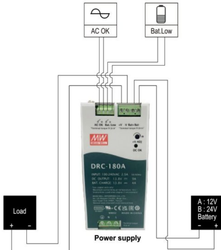
Fig 1.1 Suggested system connection
