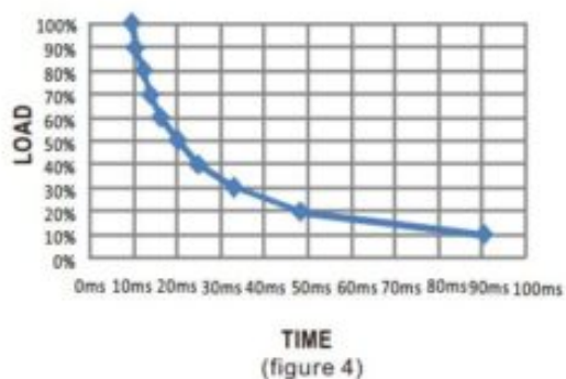
DDR-240C-48
