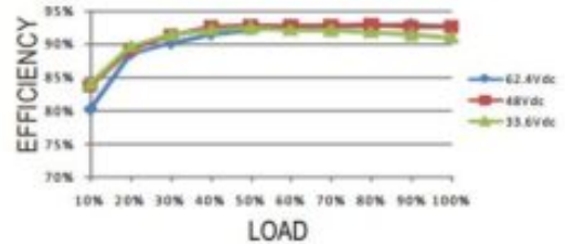
DDR-240C-48
