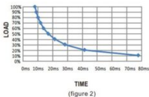
DDR-240C-48
