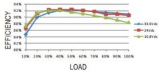
DDR-240B-48
