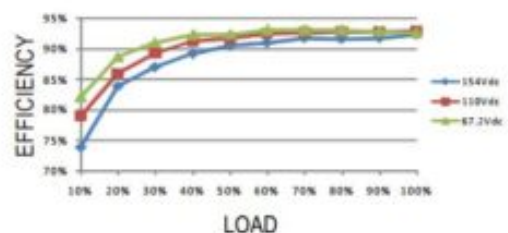
DDR-240D-48
