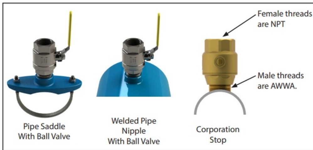
Figure 6. Installation Valve Options
