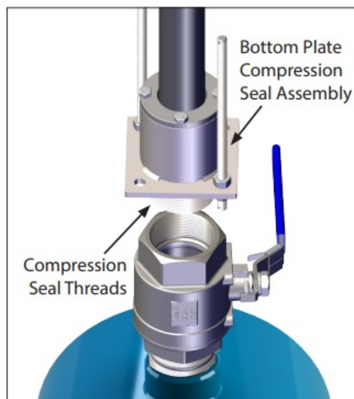
Figure 7. Sensor Installation
