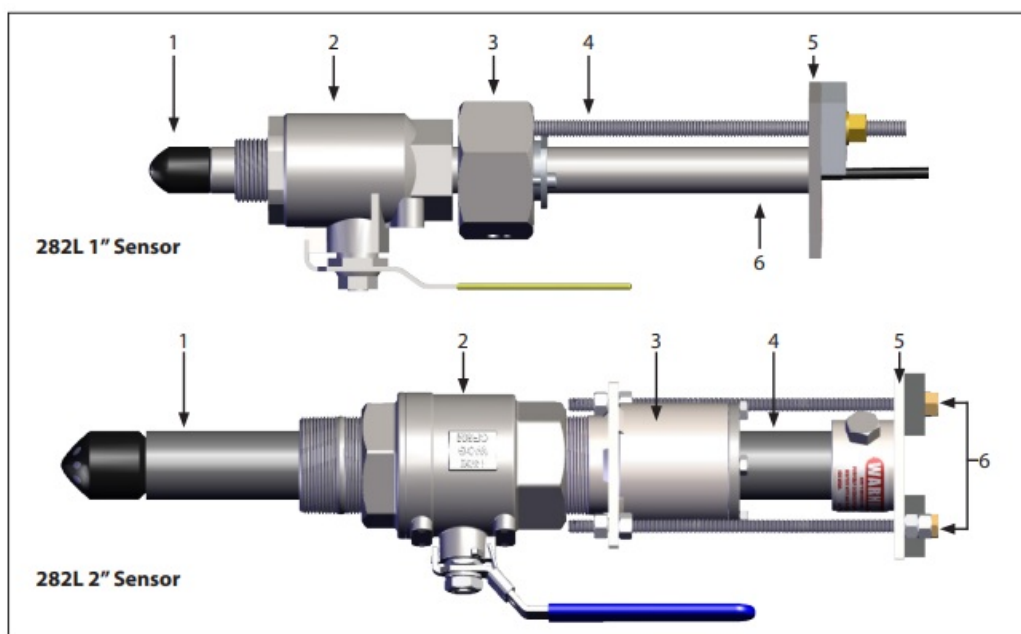
Figure 4. Parts Diagrams
