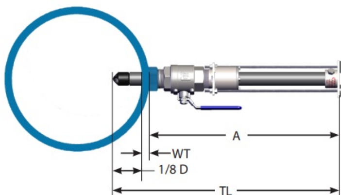
Figure 10. 1/8 ID Position
