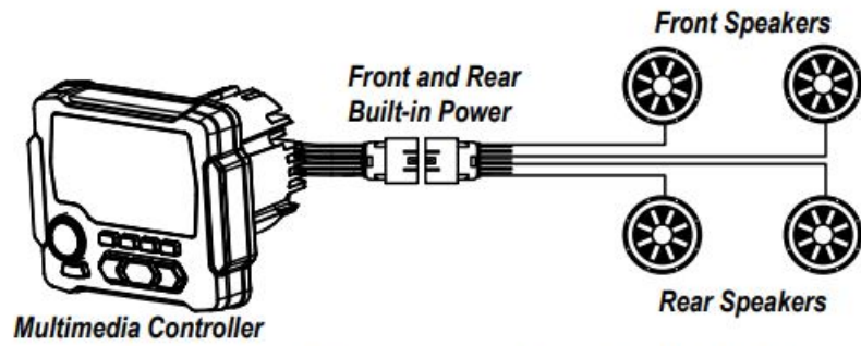
4-Speaker System using Built-in Power
