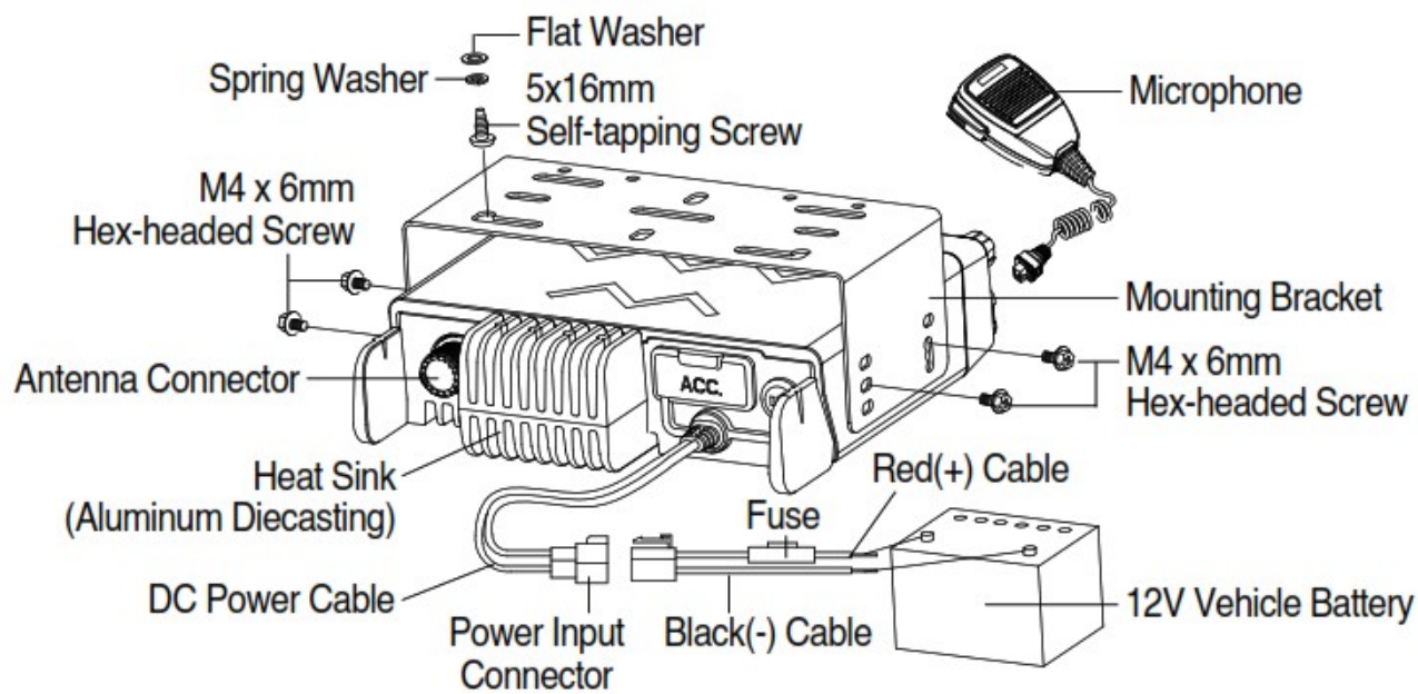
Figure 4-1) Parts & Installation
