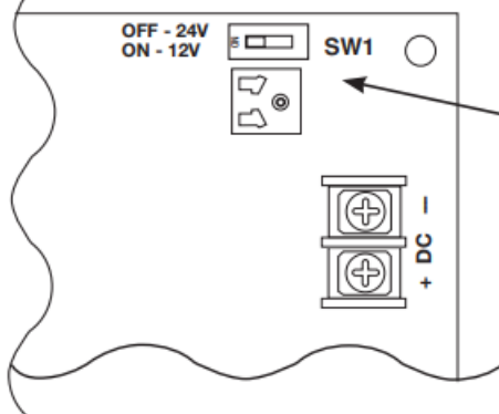
Fig. 1a - AL400ULXB2 / AL600ULXB Power Supply Board
