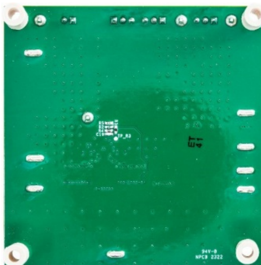
Figure 2. MAX42403 EV Kit Board Photo—Bottom
