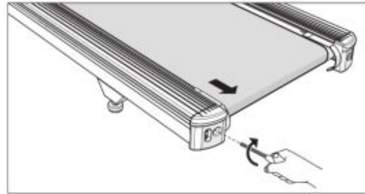
TIGHTENS LEFT SIDE OF ROLLER
