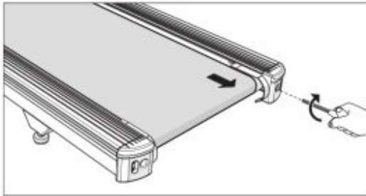
TIGHTENS RIGHT SIDE OF ROLLER
