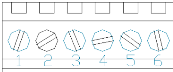
Figure 13: RS422 Header
