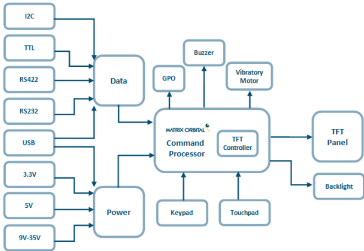
Figure 2: Functional Diagram
