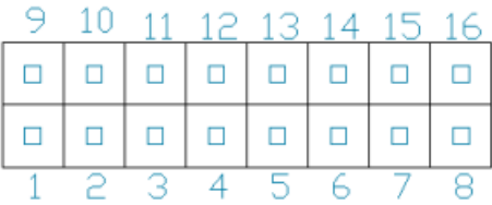
Figure 15: GPO Header
