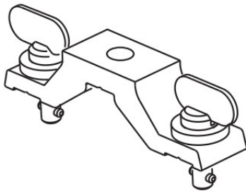
Martin standard omega bracket: P/N 91602001
