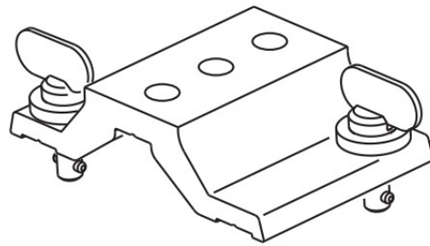
Martin 250-300 wide omega bracket: P/N 91602000
