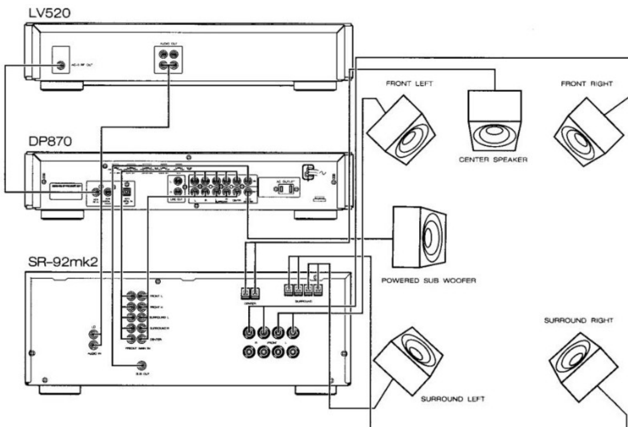
Connection diagram (LV520/DP870/SR-92mk2)
