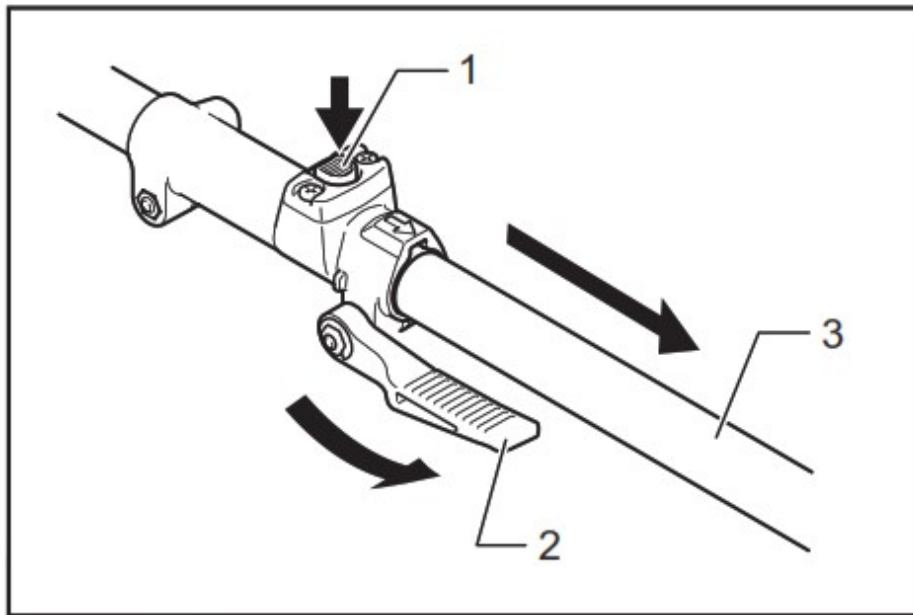
► 1. Release button 2. Lever 3. Pipe
