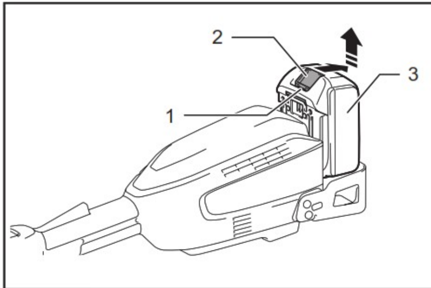
► 1. Red indicator 2. Button 3. Battery cartridge
