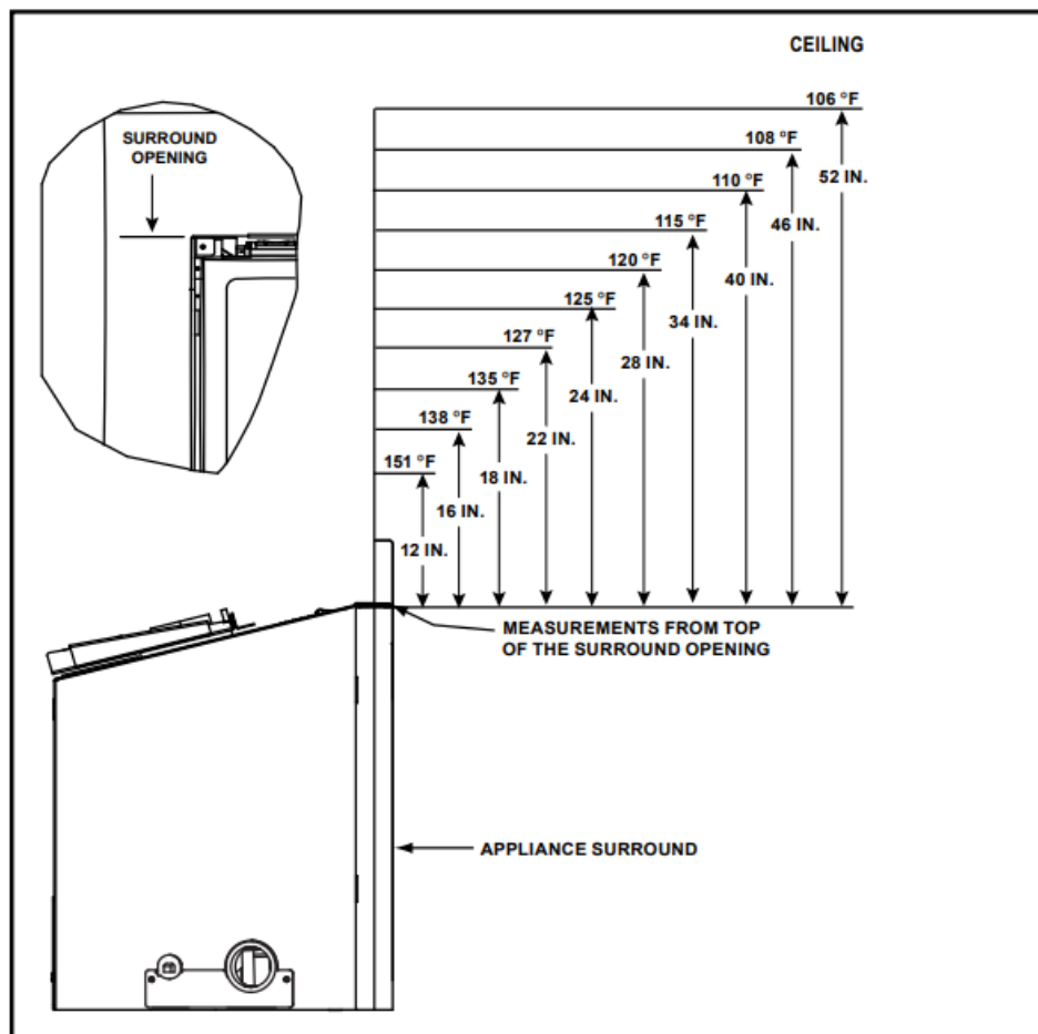
Figure 3.3 Good Faith Wall Surface Temperatures Above Appliance
