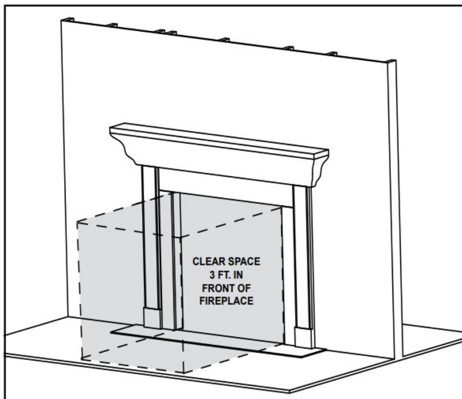
Figure 3.1 Clear Space Requirement - All Models
