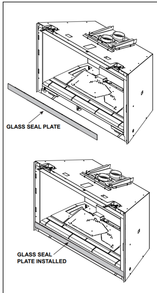
Figure 4.3 Glass Seal Plate
