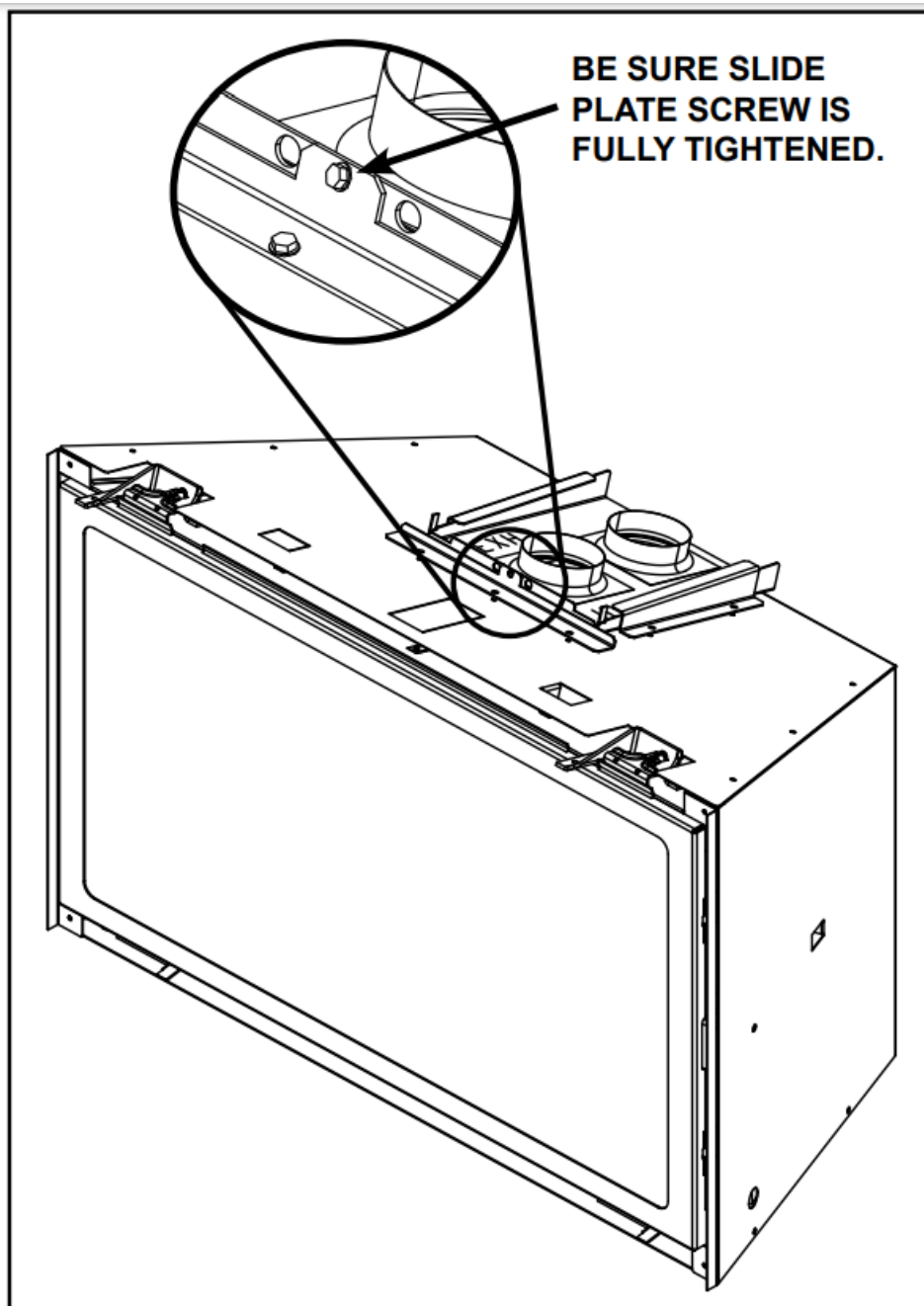
Figure 3.5 Collar slide Plate Screw Detail
