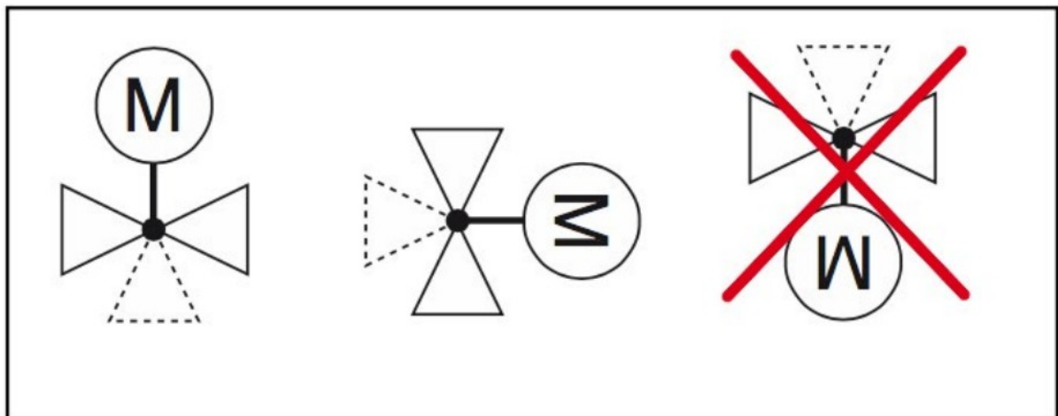
Installing the Radio Small Actuator
