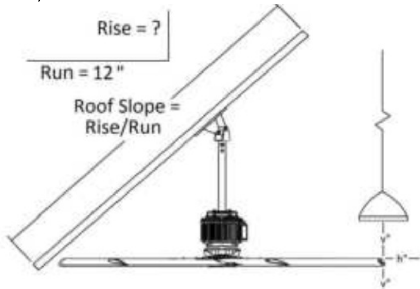
Figure 2: Fan Clearance (h/v see Fig 4) Note: Guy wires not shown.
