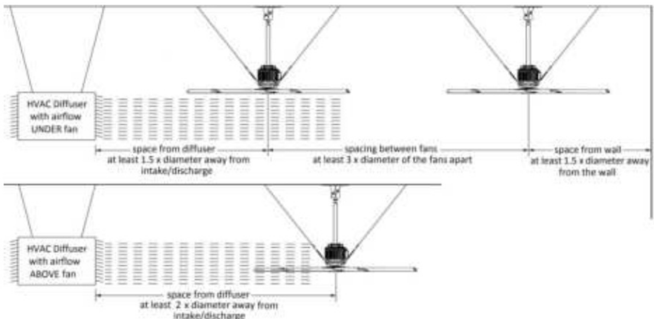
Figure 1: Fan Clearance and Placement
