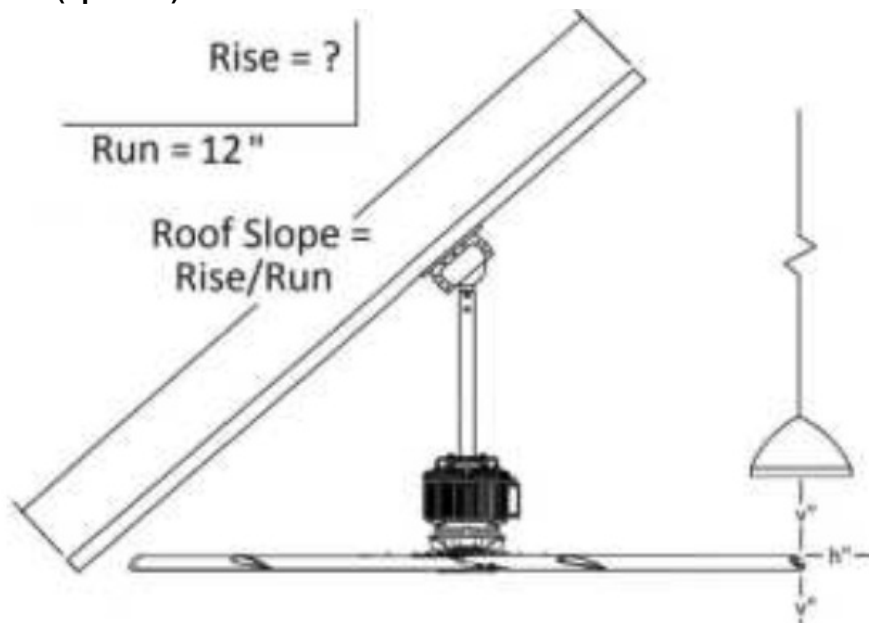
Figure 5: Fan Clearance (h/v see Fig 7)
