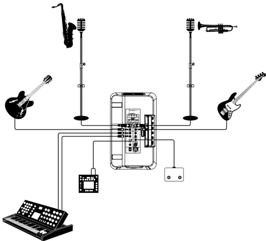
SHOWBOX BATTERY POWERED ALL-IN-ONE PERFORMANCE RIG WITH BREAKAWAY MIX CONTROL
