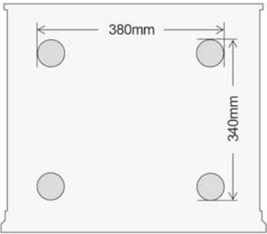
Insulator position / dimensions
