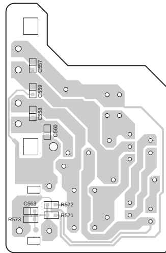
Soldering side
