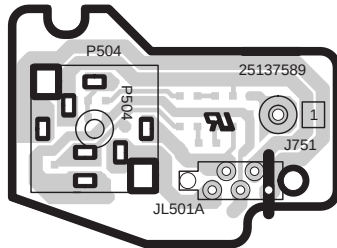
Component side
