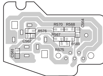
Soldering side
