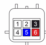
6 pins JST male connector contact insertion view
