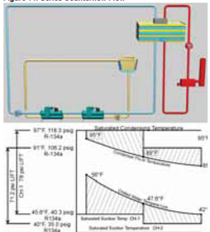
Figure 14: Series Counterflow Flow
