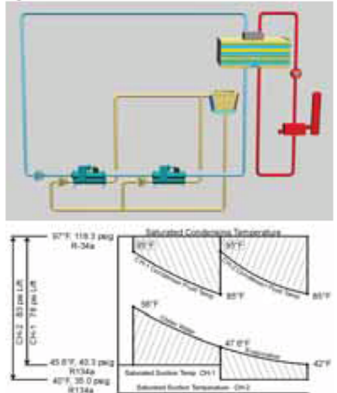
Figure 13: Series Parallel Flow
