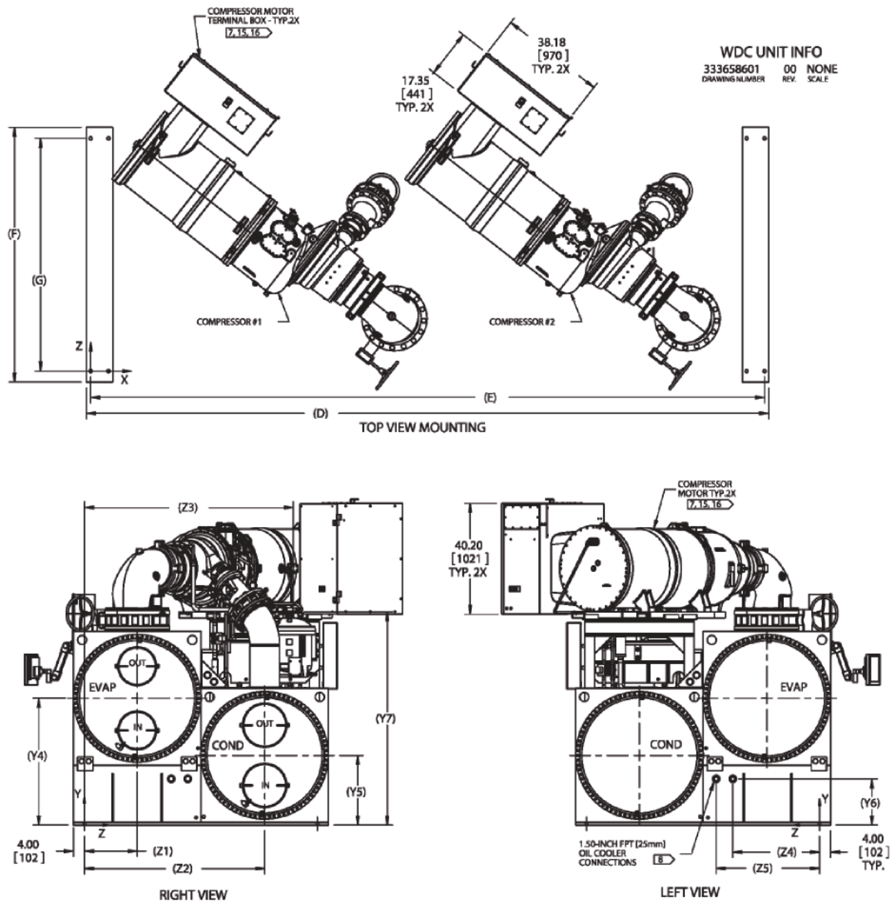
Figure 31: WDC 100/113/126 (Higher Voltage Models - 10/11kV only) continued
