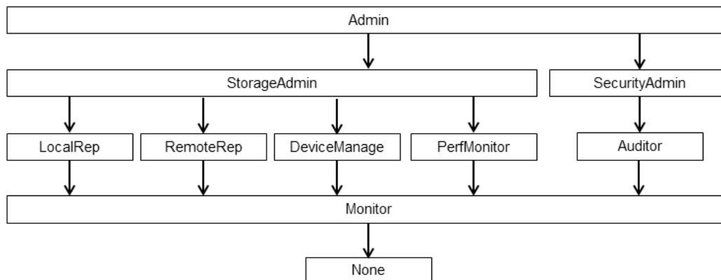
Figure 28. Hierarchy of user roles
