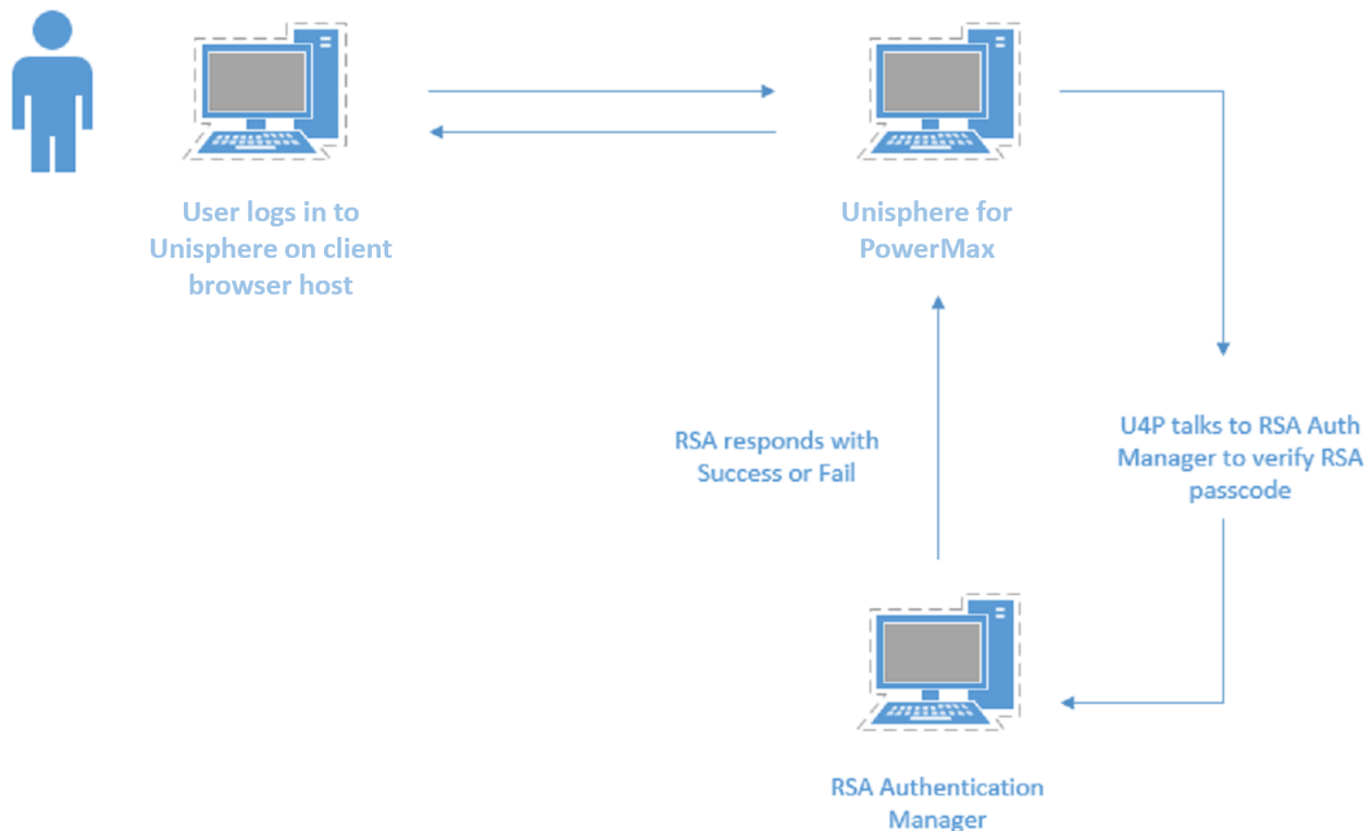
Figure 27. Overview of Multi-factor authentication for SecurID
