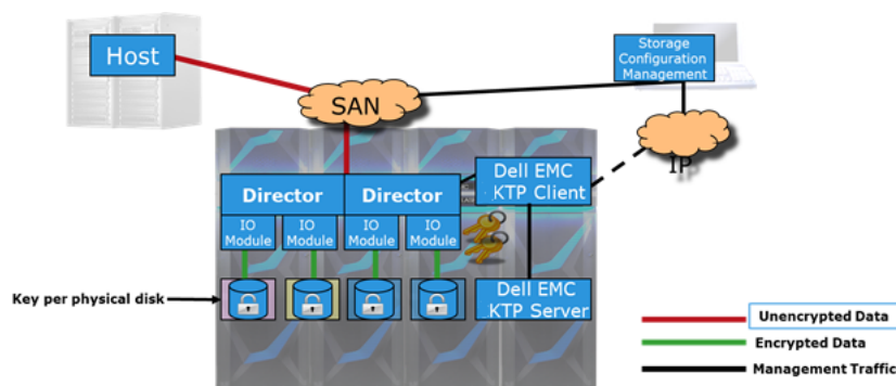
Figure 1. D@RE architecture for PowerMaxOS 5978 and earlier
