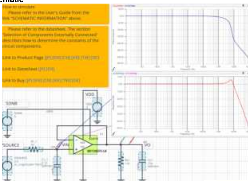
Figure 1. Simulation Schematic
