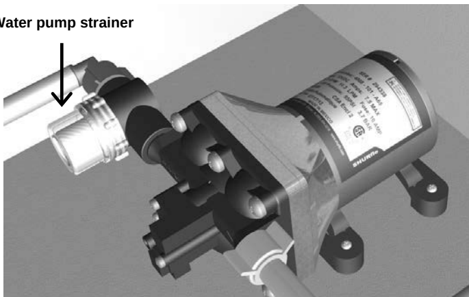
Water pump
