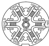
7-way trailer plug - Car end, rear view
