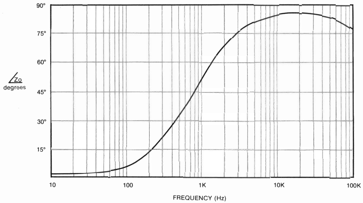
Fig. 2.9 Nominal Output Phase Angle
