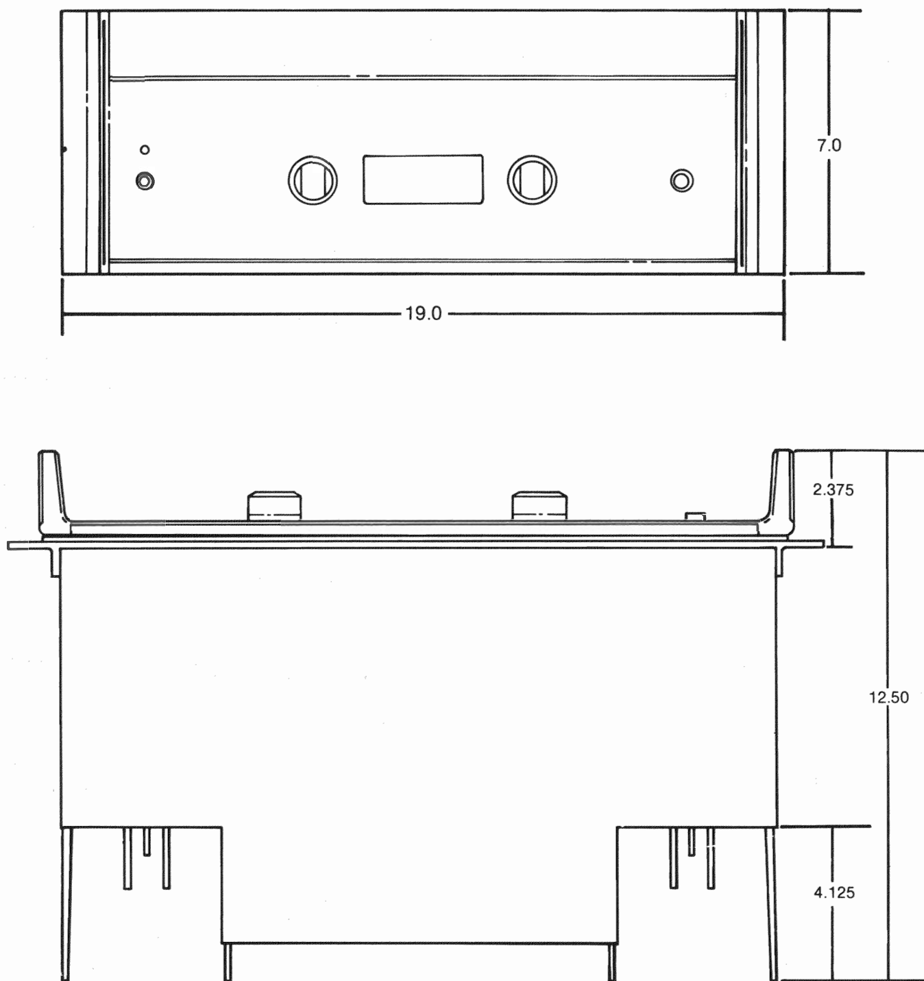
Fig. 3.1 Power Line Four Mounting Dimensions
