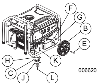
Figure 2-10. Wheel & Foot Assembly
