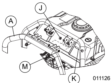
Figure 2-11. Handle Assembly
