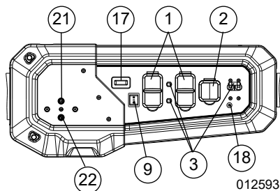
Figure 2-2. Control Panel (Rocker Switch Electric Start)
