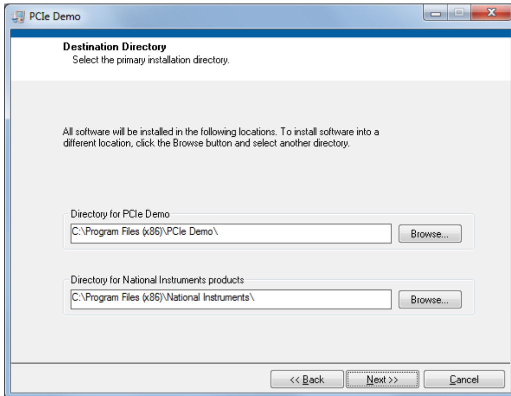
Figure 15 • GUI Installation
