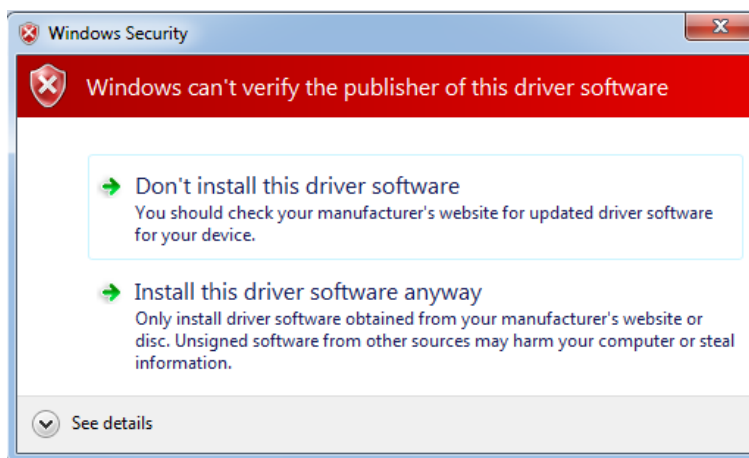
Figure 14 • Windows Security
