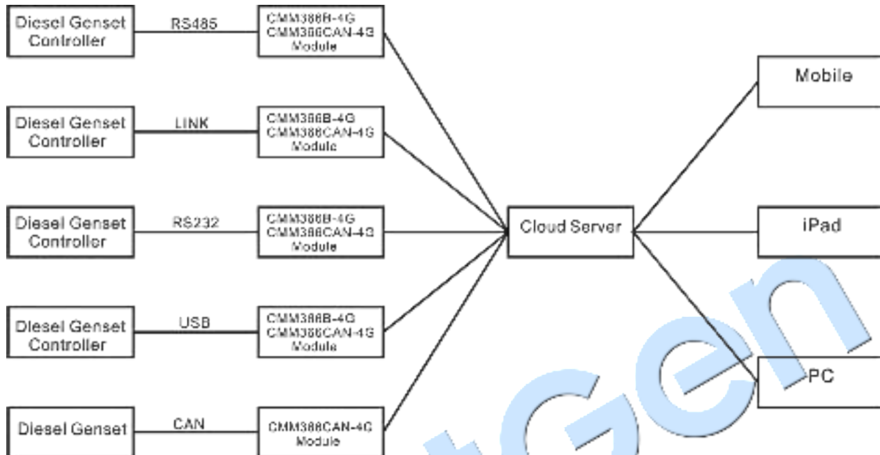
Fig.13 – CMM366B-4G/CMM366CAN-4G System Application Diagram
