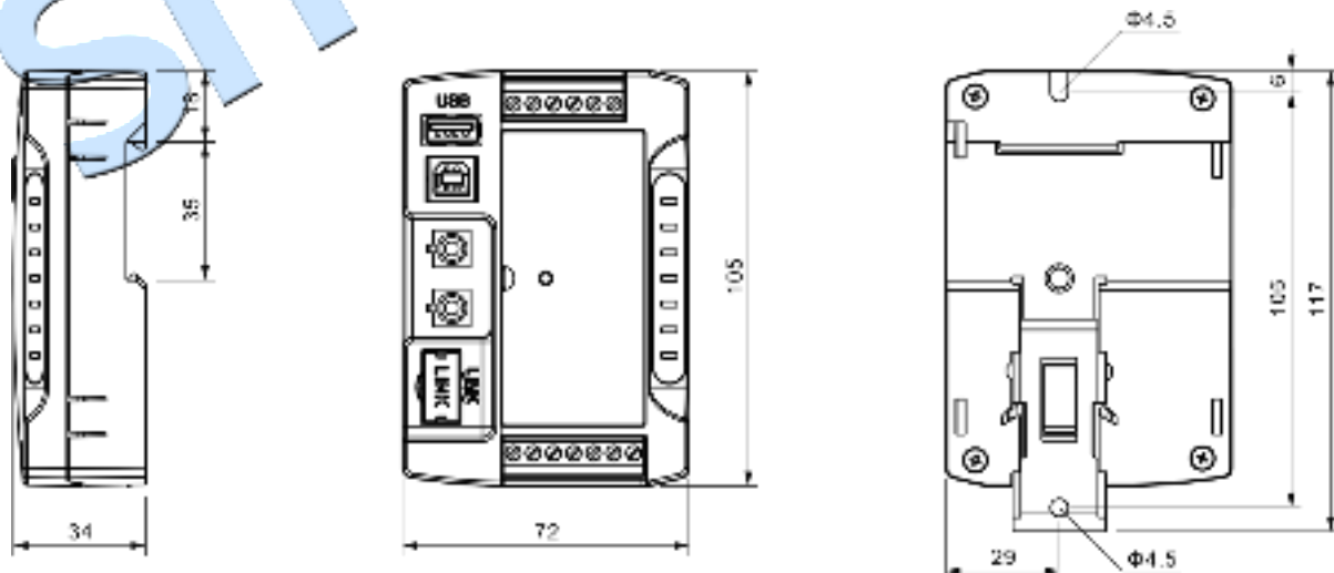
Fig.14 – CMM366B-4G/CMM366CAN-4G Case Dimension
