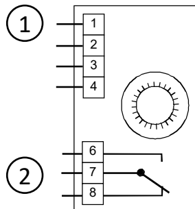
Figure 3 Wiring.
