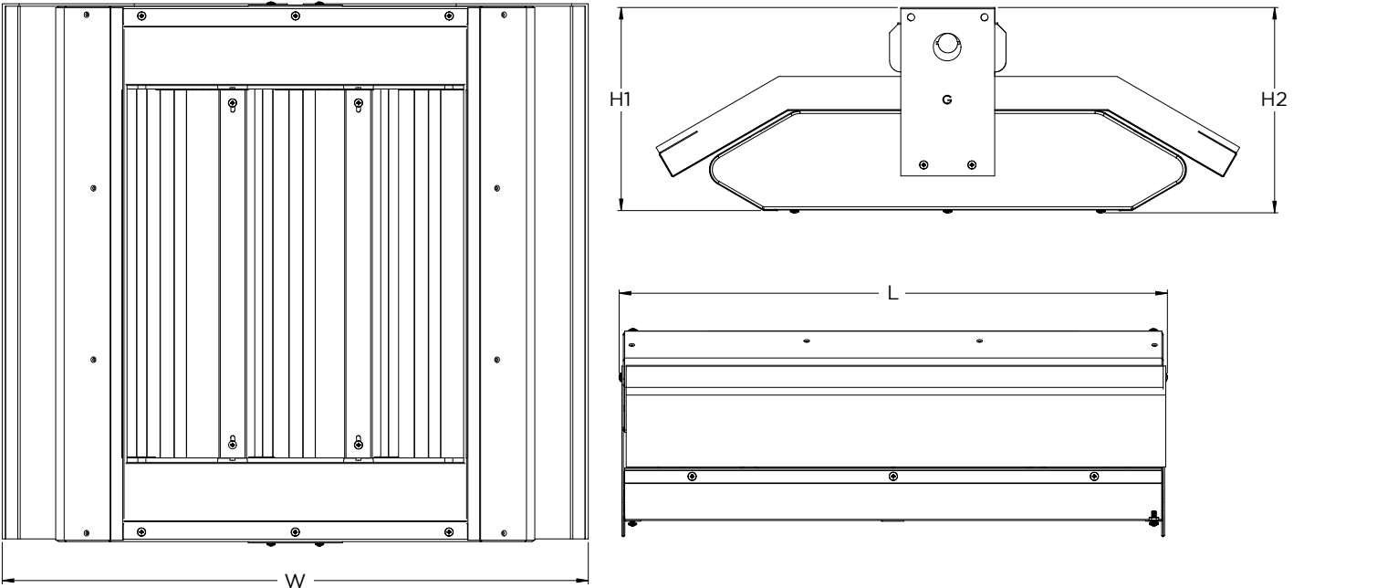
Dimensions: 3-Element
