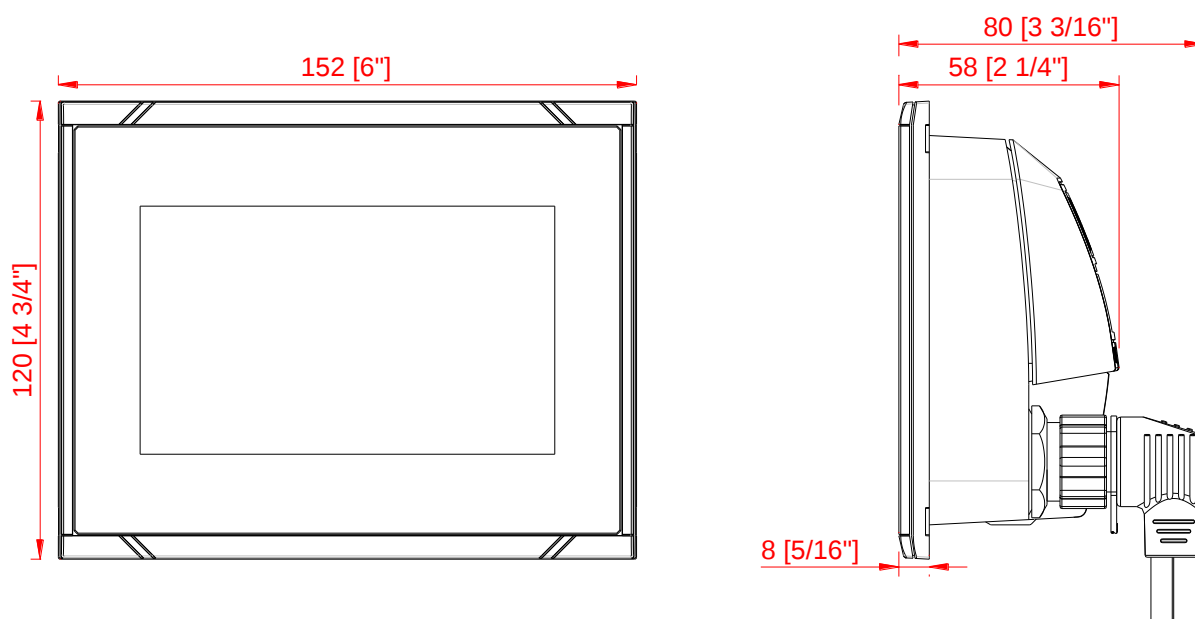
Figure 3. Dimensions
