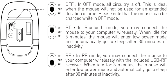
Fig. 01 / Mouse Switch
