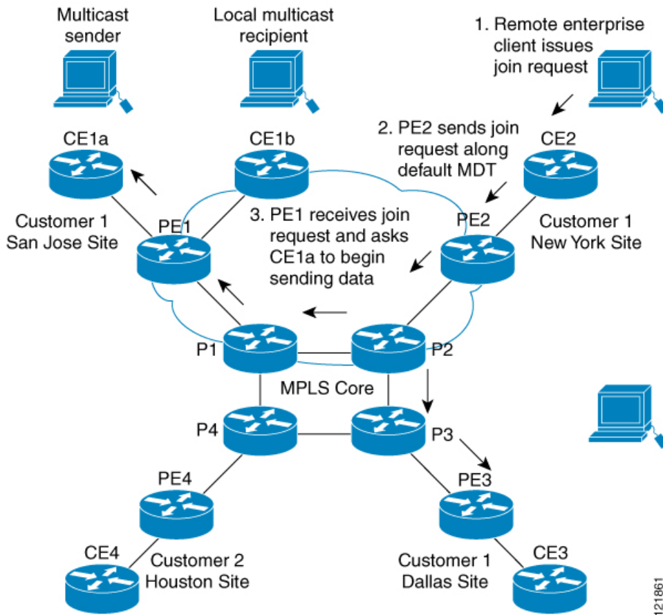
Figure 25: Initializing the Data MDT
