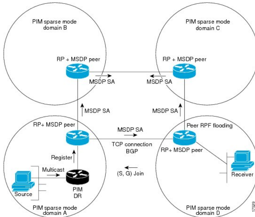
Figure 19: MSDP Running Between RP Peers
