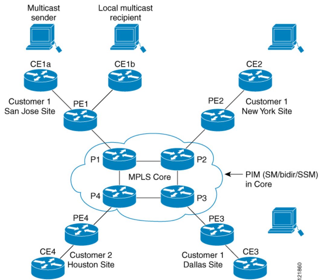
Figure 24: Default Multicast Distribution Tree Overview
