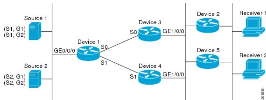
Figure 35: ECMP Multicast Load Splitting and the PIM Assert Process in PIM-SM and PIM-SSM
