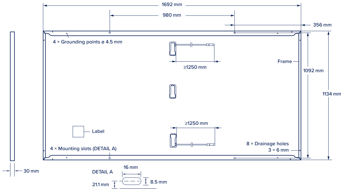
Fig. 1: External dimensions and components for Q.PEAK DUO M-G11 Q.PEAK DUO M-G11+ Q.PEAK DUO BLK M-G11 Q.PEAK DUO BLK M-G11+
