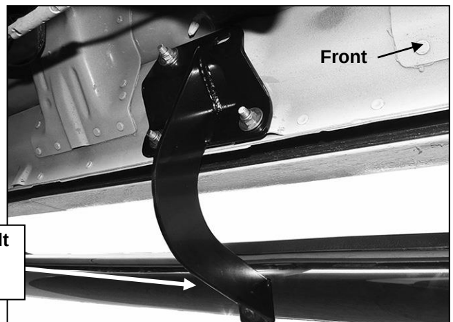
(Fig 7) Driver side center Bracket installation
