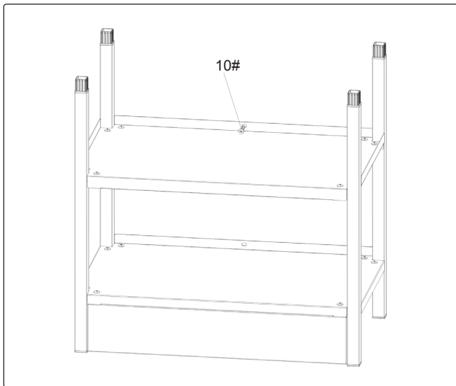
Step 7. Fix cabinet to the wall using self-tapping screw ST4.8*30.
